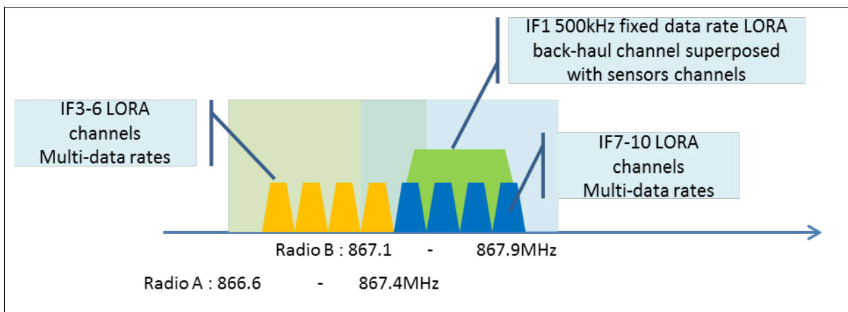
Figure 10 Radio Spectrum
